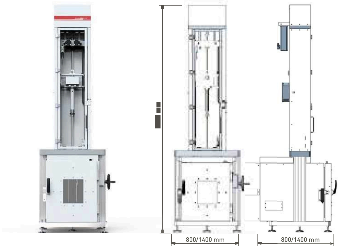
Dimensions with climatic chamber
